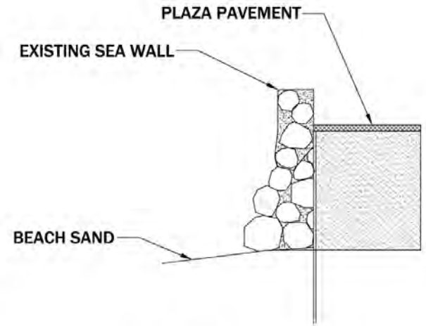
SEA WALL RESTORATION DETAIL SECTION
